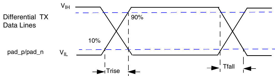
Figure 23. Rise/fall time
